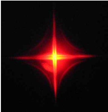
Fig. 6 Optical pattern generated by the micra-pyramid patterns under the normal incident illumination of a 633nm HeNe laser
